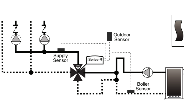
4-way Valve with Low Temperature Zones
