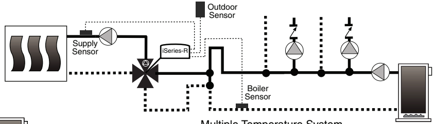
Multiple Temperature System
