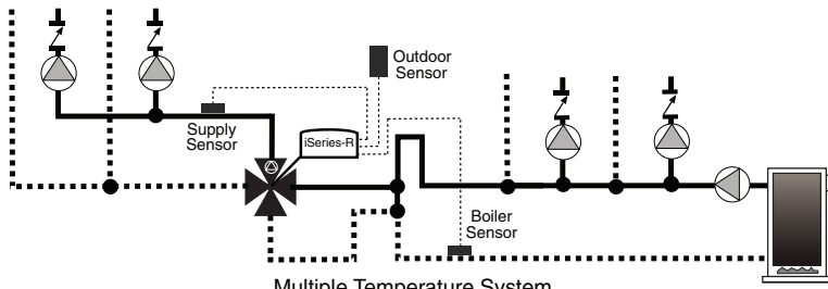
Multiple Temperature System
